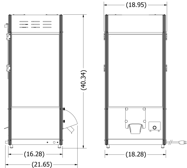
Drawing shown for dimension reference only.
